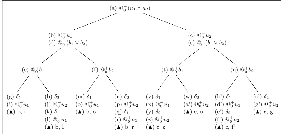
Fig. 3. Default tableau for u_1 \wedge u_2 from \{\{b_1 \vee b_2\}, \{\top \xrightarrow{u_i \wedge \neg b_i} u_i \mid i \in \{1, 2\}\}\} .
